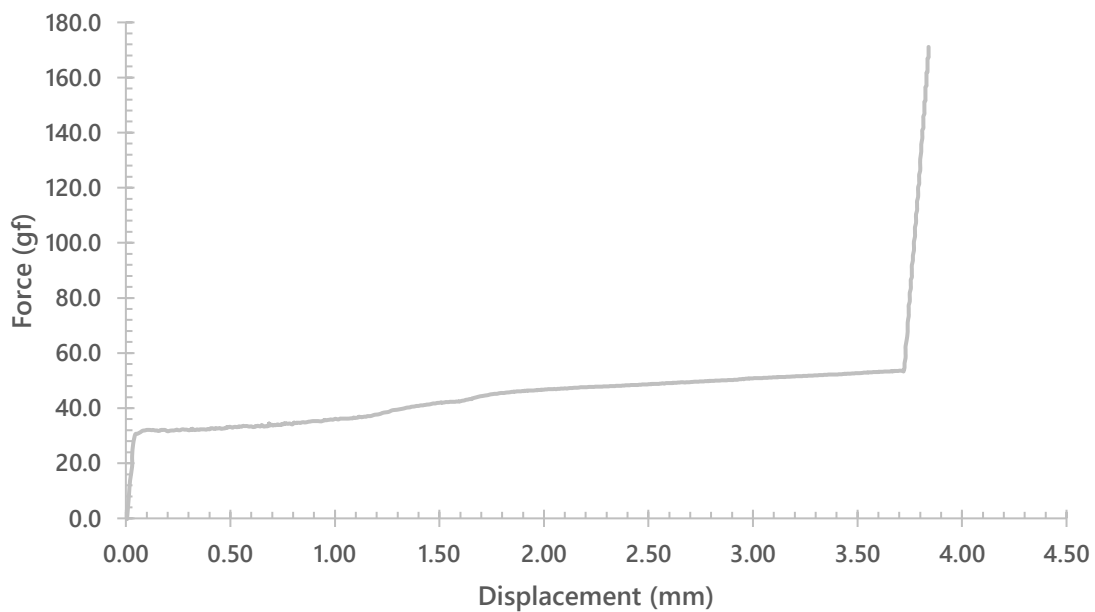
HMX Dirty Pink (57g) (Upstroke)
